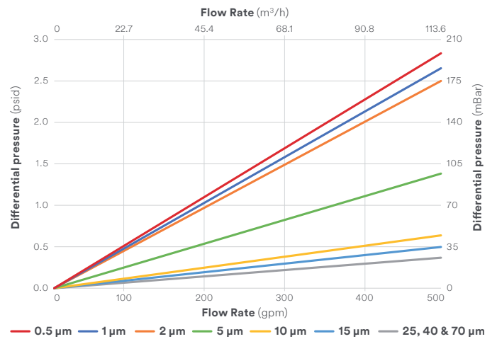
60" HF flow rate vs differential pressure
