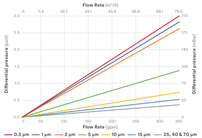
40" HF flow rate vs differential pressure
