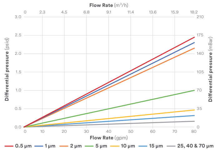
10" HF flow rate vs differential pressure
